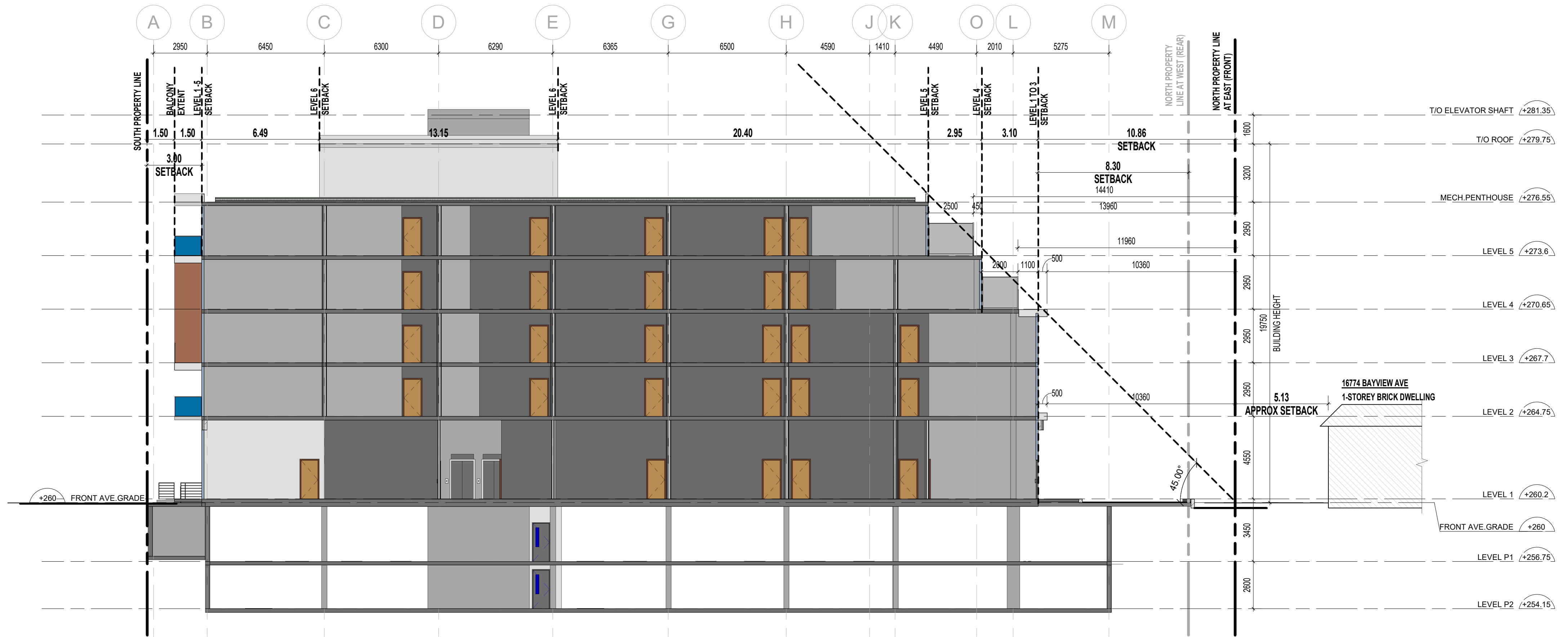
1 SCHEMATIC BUILDING SECTION 1 A4.01 SCALE: 1 : 150
