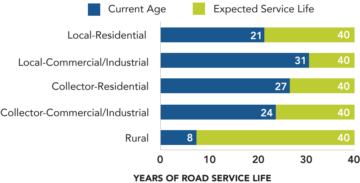
AVERAGE AGE AND EXPECTED SERVICE LIFE OF ROADS
